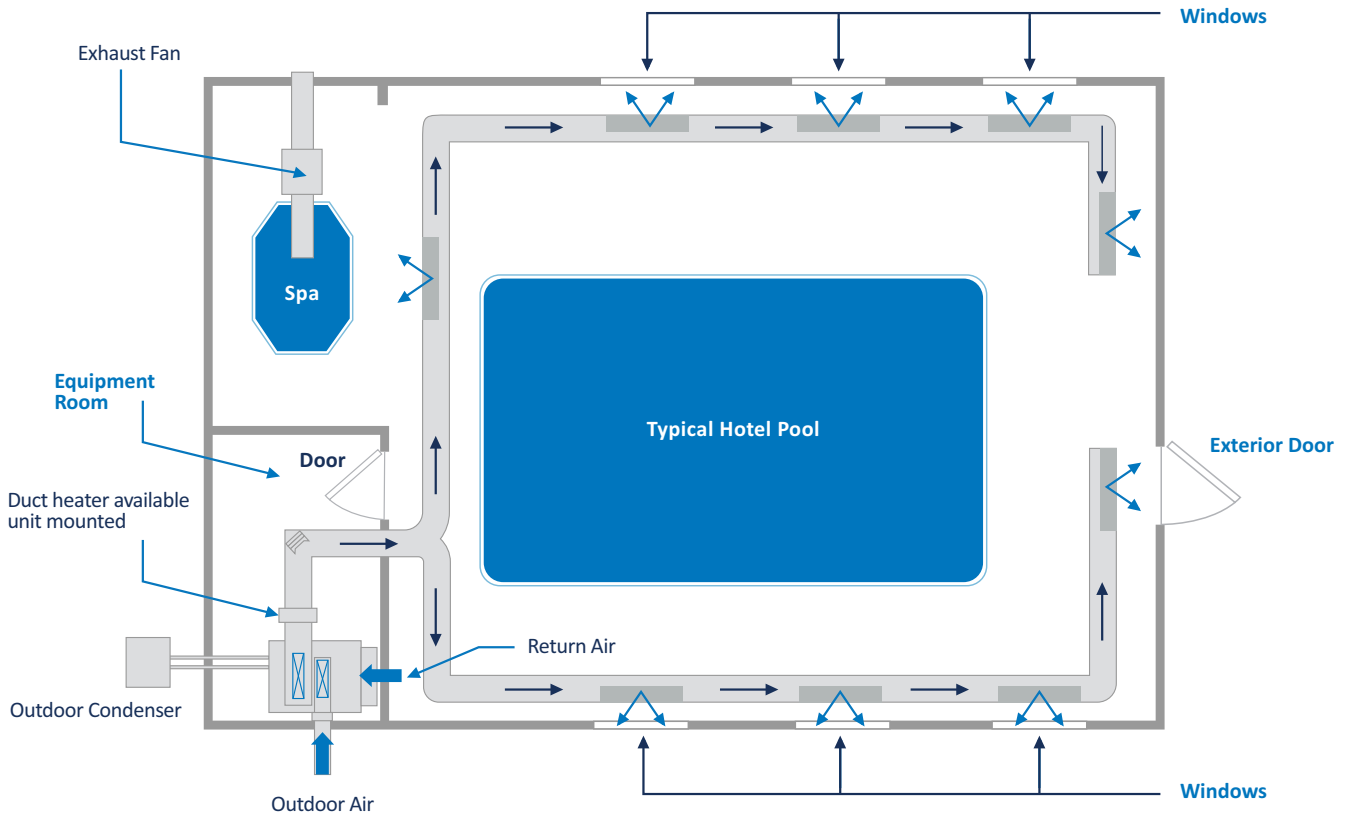
FIGURE 13: TYPICAL HOTEL AND THERAPY POOL LAYOUT
