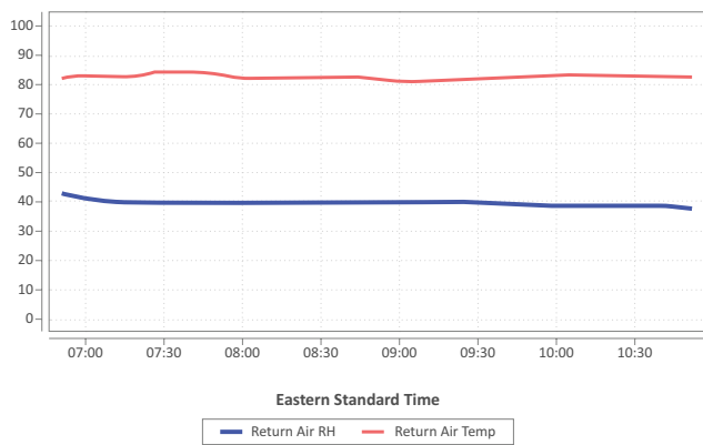
FIGURE 19: SERESCO'S MODULATING REHEAT SYSTEM PROVIDES STABLE TEMPERATURES AND RH LEVELS
