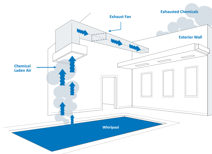
FIGURE 3: EXHAUST AIR
