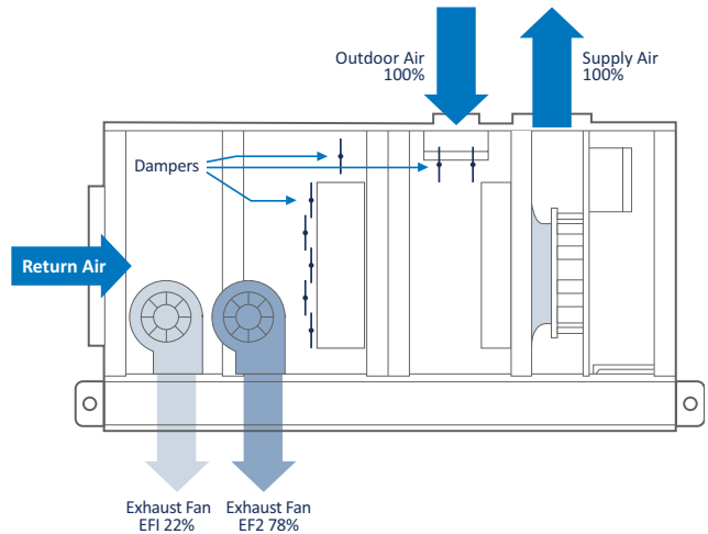
FIGURE 16: PURGE-ECONOMIZER MODE
