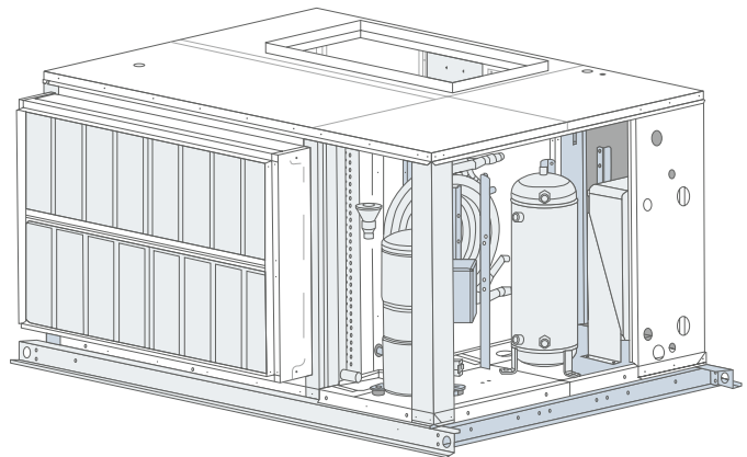
FIGURE 12: SLB CABINET
