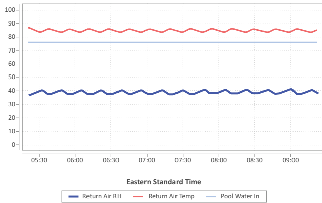
FIGURE 18: HOT GAS REHEAT COIL RESULTS IN UNSTABLE TEMPERATURES AND RH LEVELS
