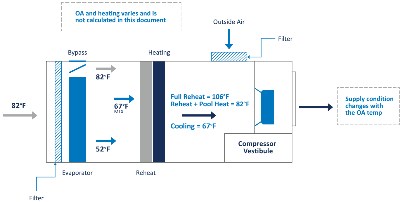
FIGURE 20: REFRIGERATION-BASED DEHUMIDIFIERS
